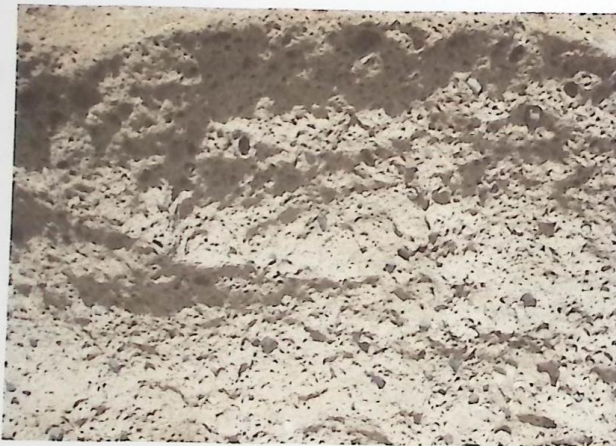
Figure 2. Photograph of a volcanic rock.
