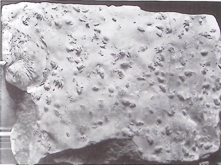
Figure 6. Bootle Museum slab number 9 showing small footprints from the lower footprint bed at Storeton.
