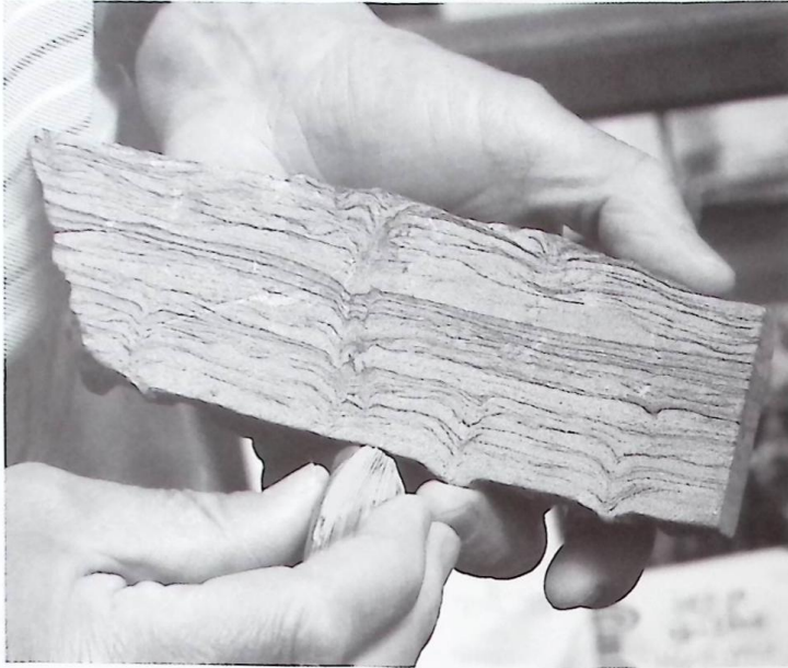
Probable escape structures, possibly produced by bivalve molluscs, seen in section perpendicular bedding. Photographed by Dr Peter Rankilor, displayed by and property of Mr Fred Owen, Manchester Geological Association.
