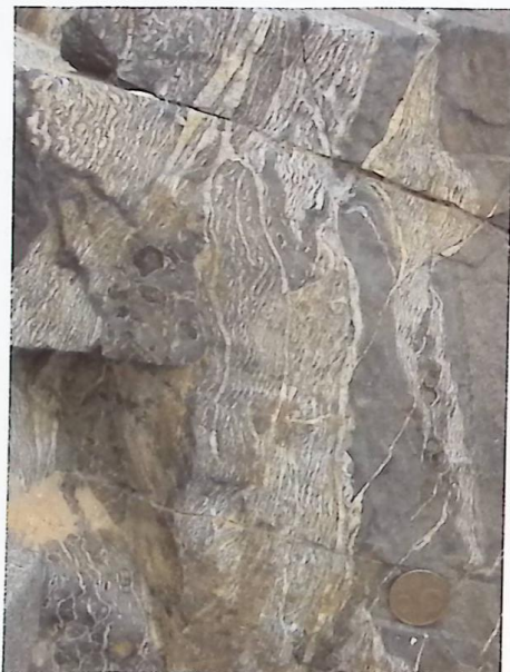
Figure 5. Sub-parallel migmatite veins, Location 2
